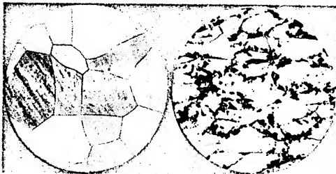
ABOVE TO LEFT —Crystalline structure of overheated, coarse-grained 14K gold. TO RIGHT —Scientifically controlled crystalline structure of Parker's 14K gold nib. The properties of these 14K golds are just as different as their photomicrographs: the first is inelastic, lifeless; the second, springy, resilient. In both views magnification is 100 diameters.
